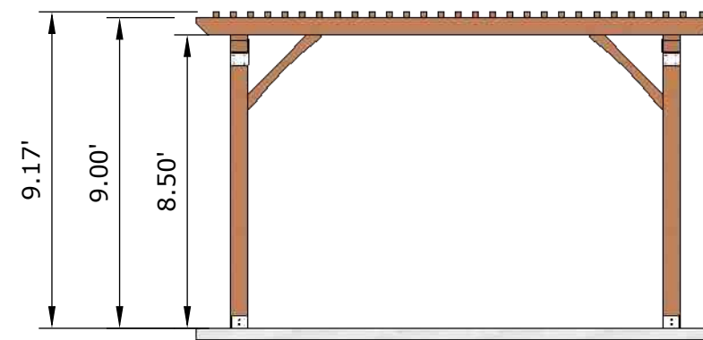
C :: Front view 001
