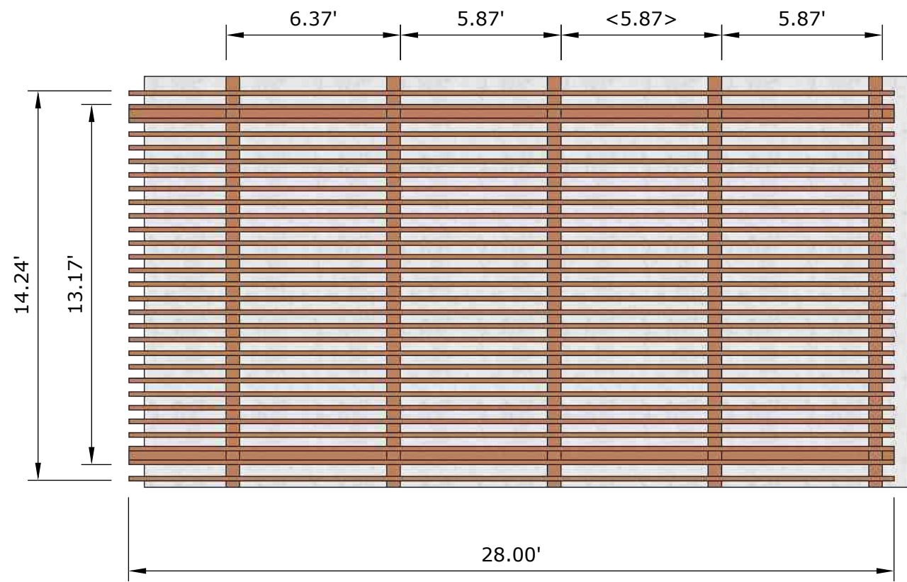
A :: Top view 001
